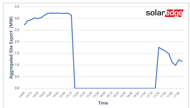
Site level curtailment on commercial site
